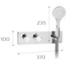
5A2805COO 3 way mixer with handset and integrated fixed bracket
