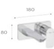
Wall-mounted basin mixer
