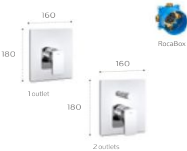
5A2B01C00 1 outlet 5A0B01C00 2 outlets 525869403 RocaBox shower valve housing unit (Required)
