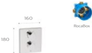
5A0C3AC00 2 outlets - Chrome 5A2C3AC00 1 outlet - Chrome 525869403 RocaBox shower housing unit (Required)
