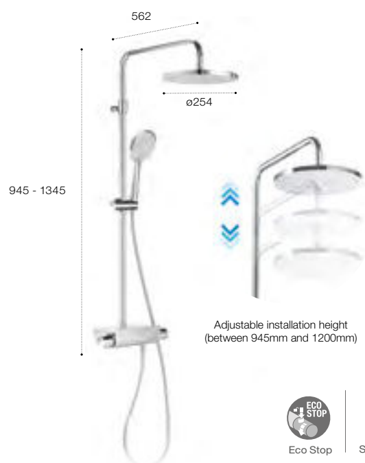
5A9788C00 Thermostatic shower column with round head
