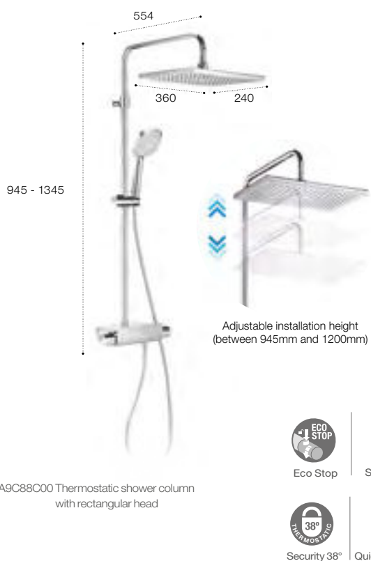
Wall-mounted shower column
