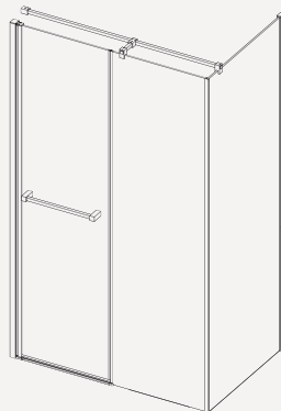
Corner configuration (600mm Door)
